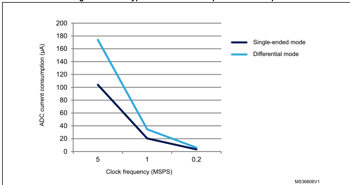
Figure 33. ADC typical current consumption on VREF+ pin
