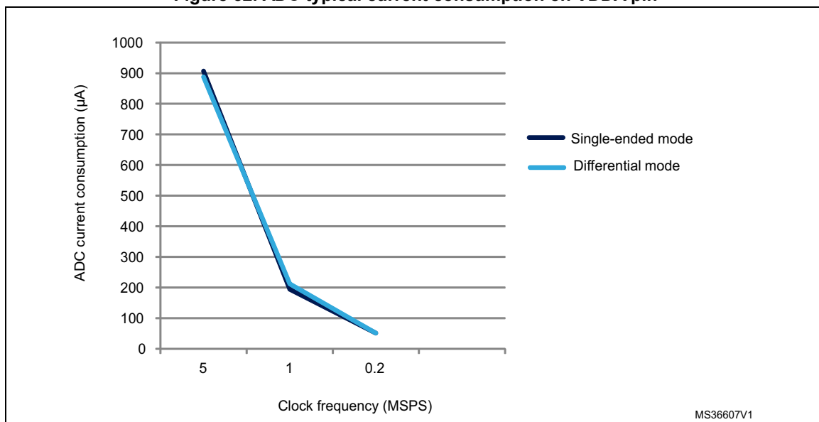
Figure 33. ADC typical current consumption on VREF+ pin
