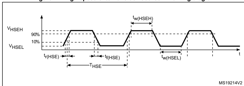
Figure 14. High-speed external clock source AC timing diagram
