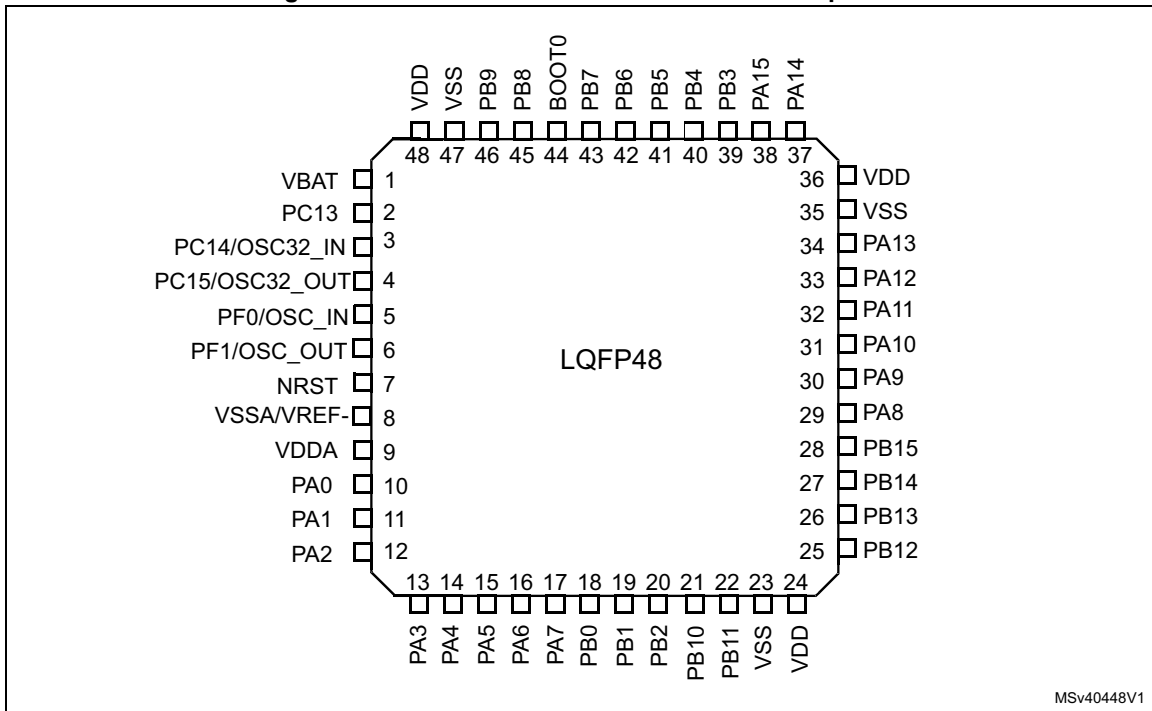
Figure 4. STM32F303xB/STM32F303xC LQFP48 pinout
