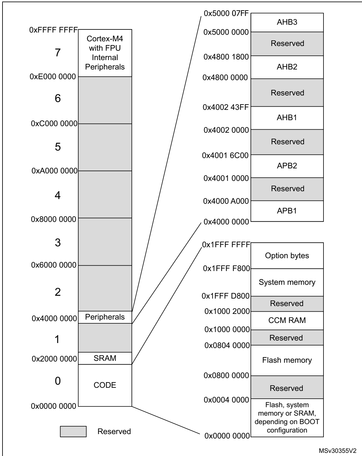
Figure 8. STM32F303xB/STM32F303xC memory map
