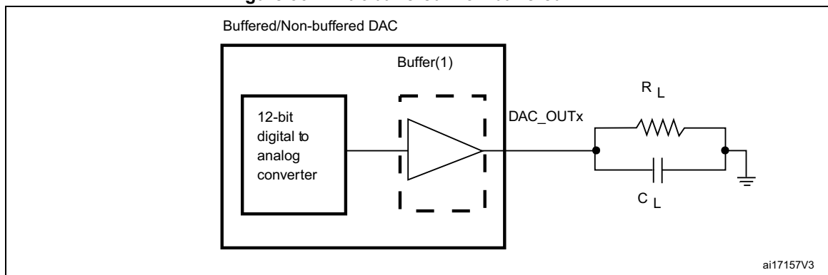
Figure 36. 12-bit buffered /non-buffered DAC
