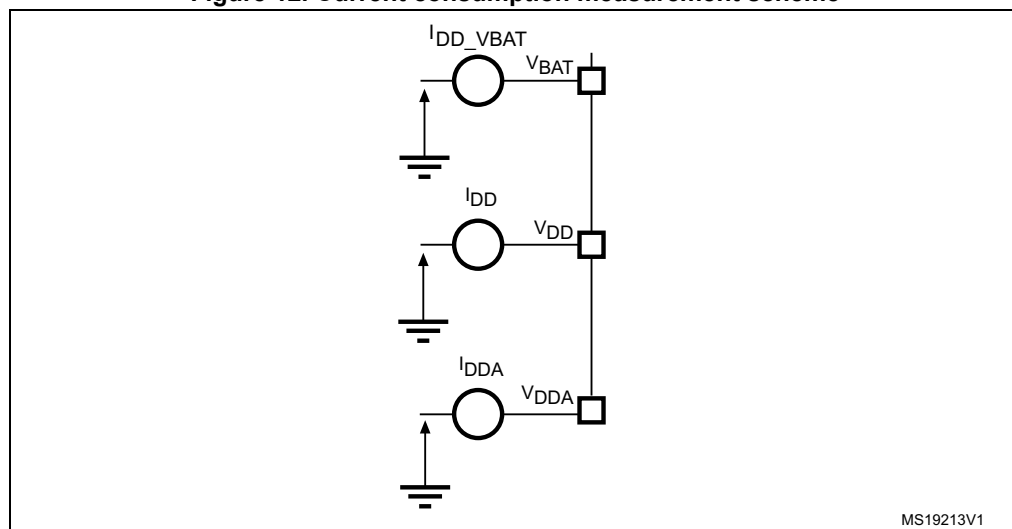
Figure 12. Current consumption measurement scheme
