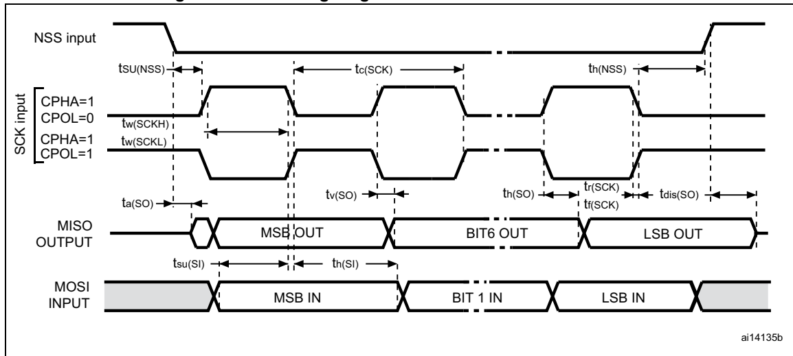
Figure 27. SPI timing diagram - slave mode and CPHA = 1 (1)
