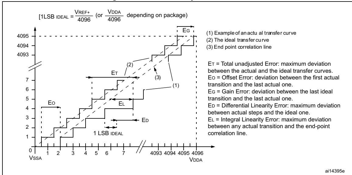
Figure 34. ADC accuracy characteristics
