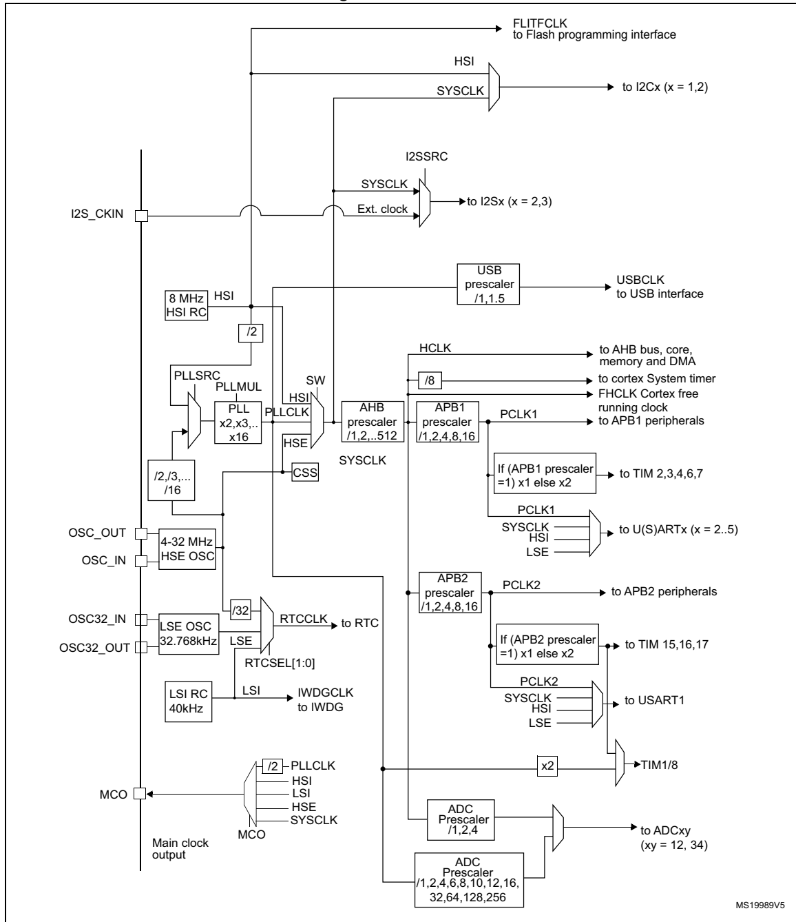
Figure 2. Clock tree
