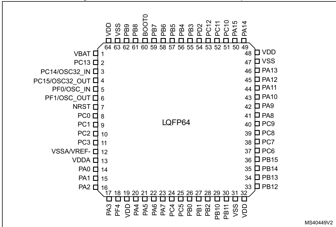
Figure 5. STM32F303xB/STM32F303xC LQFP64 pinout
