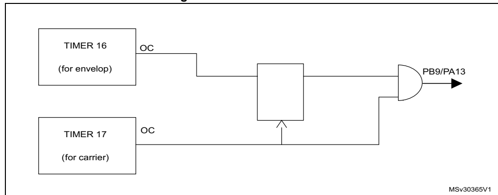
Figure 3. Infrared transmitter
