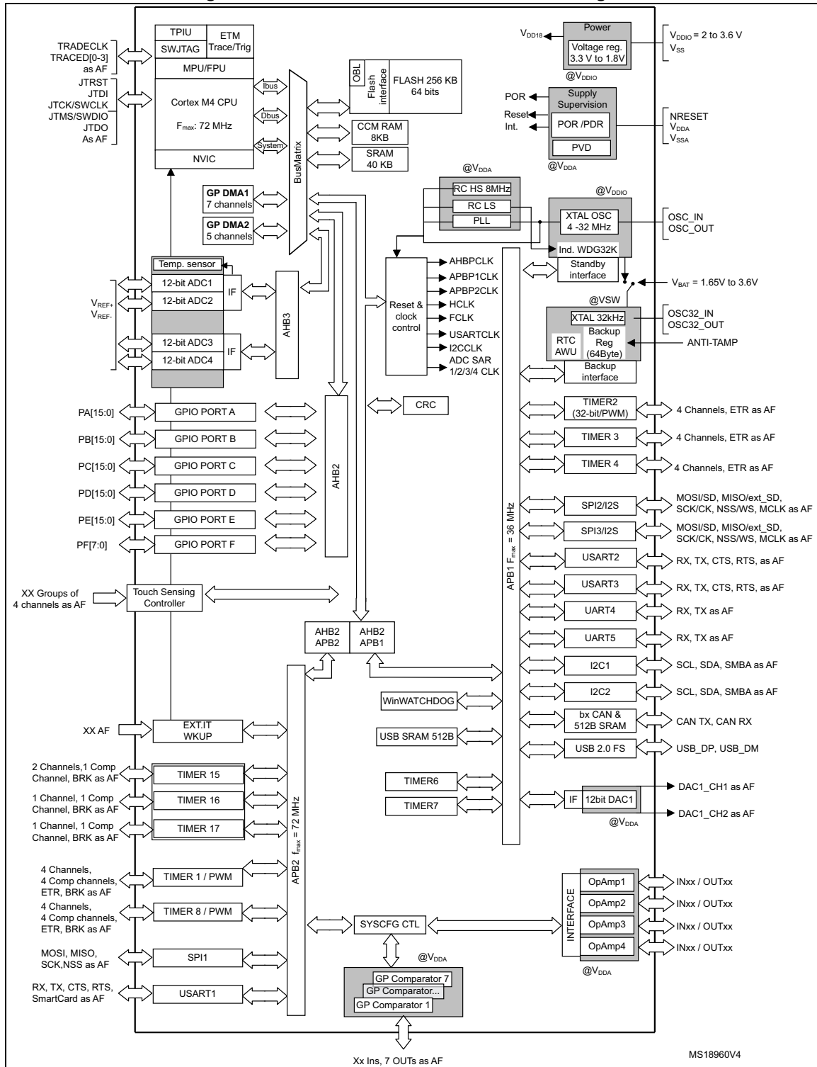
Figure 1. STM32F303xB/STM32F303xC block diagram
