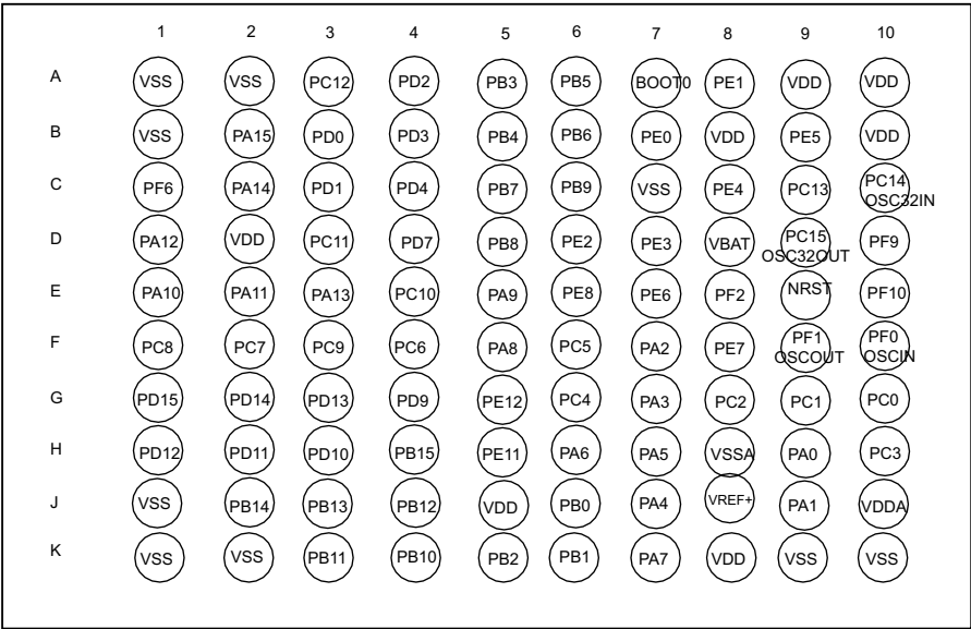
Figure 7. STM32F303xB/STM32F303xC WLCSP100 pinout
